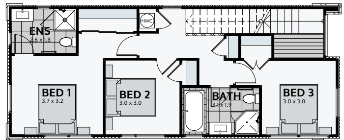
FIRST FLOOR
